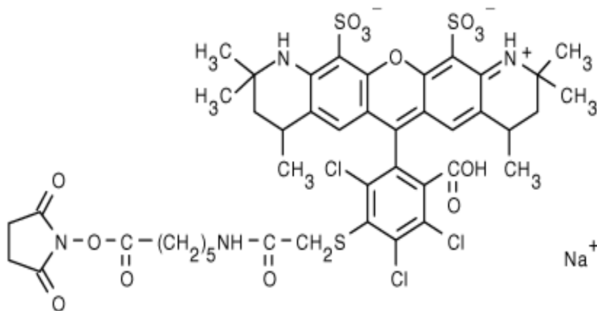
e.g. AlexaFluor 546
